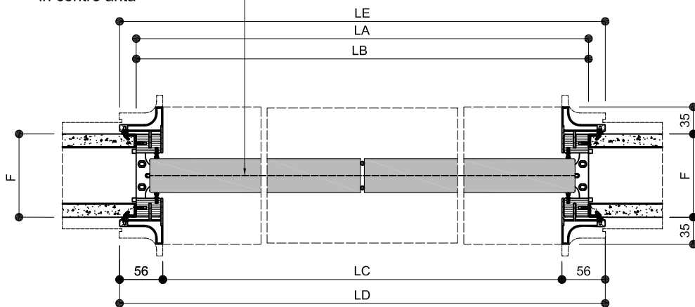
MISURE STANDARD (mm)
